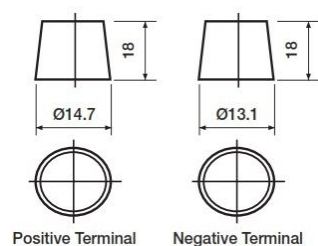
Positive Terminal
